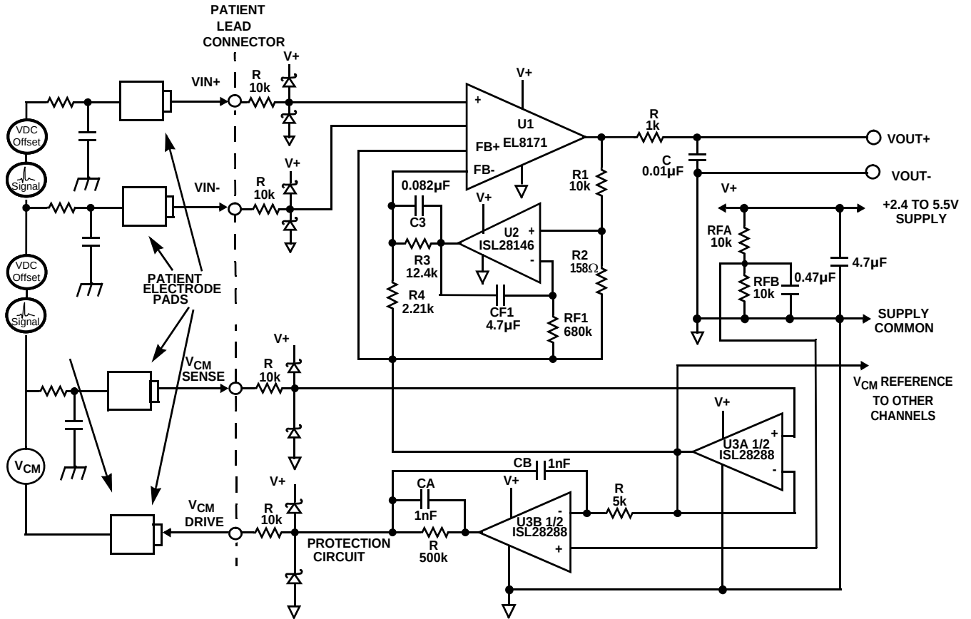
FIGURE 38. ECG/EEG AMPLIFIER
