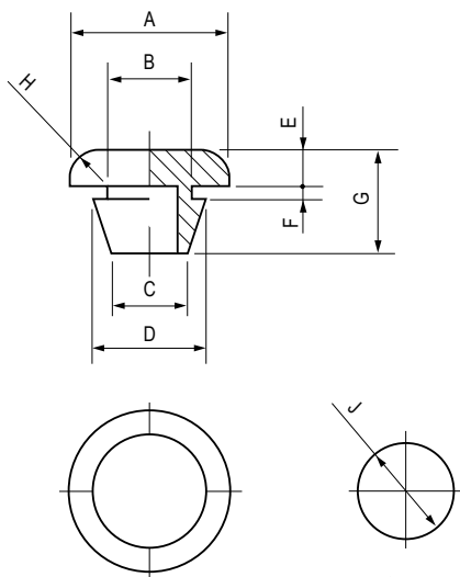
取付穴図 Hole for Installation
