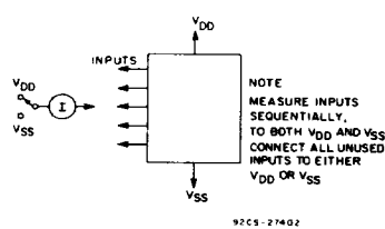
Fig. 15 - input-leakage current.
