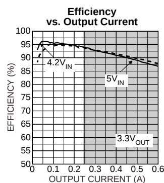
Figure 2. Efficiency Curve
