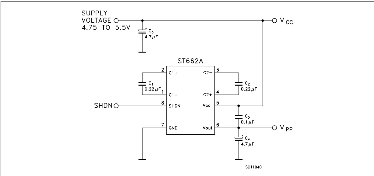
Figure 16. Electrical schematic
