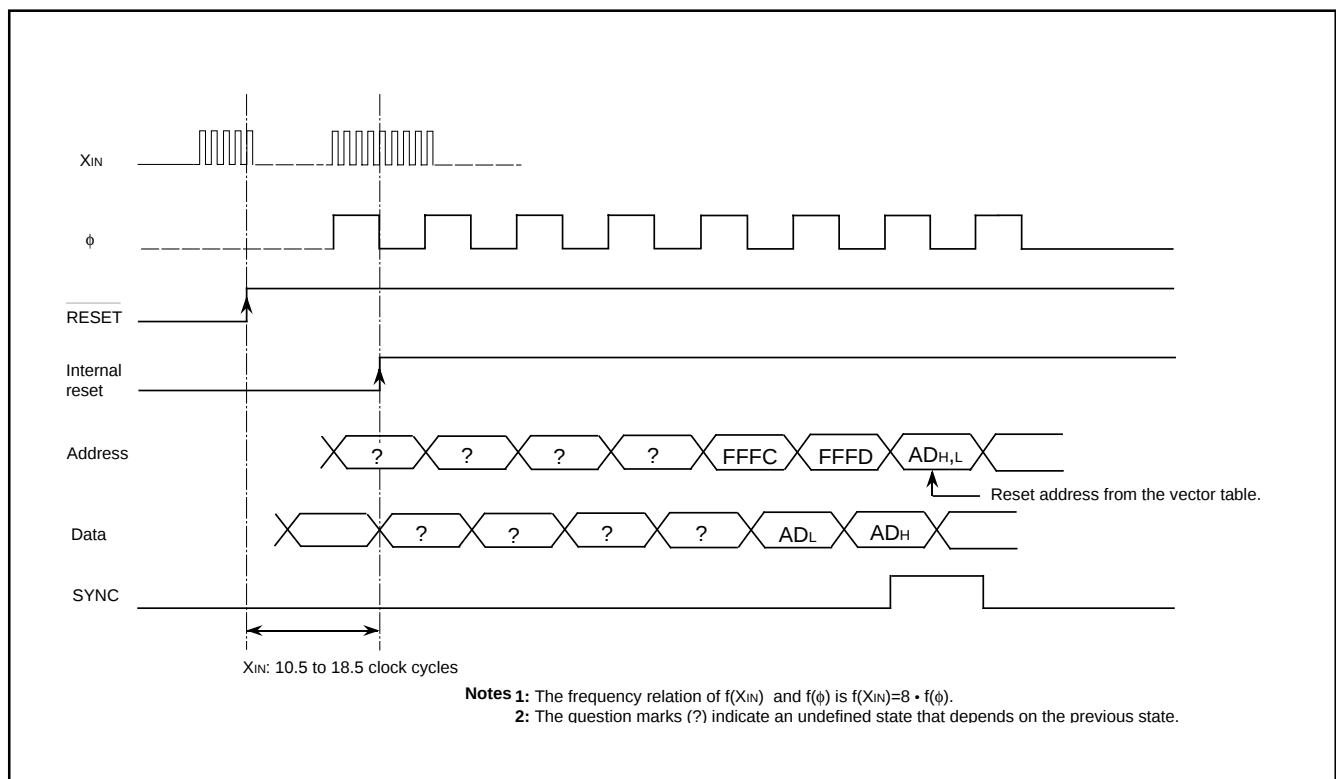
Fig. 79 Reset sequence
