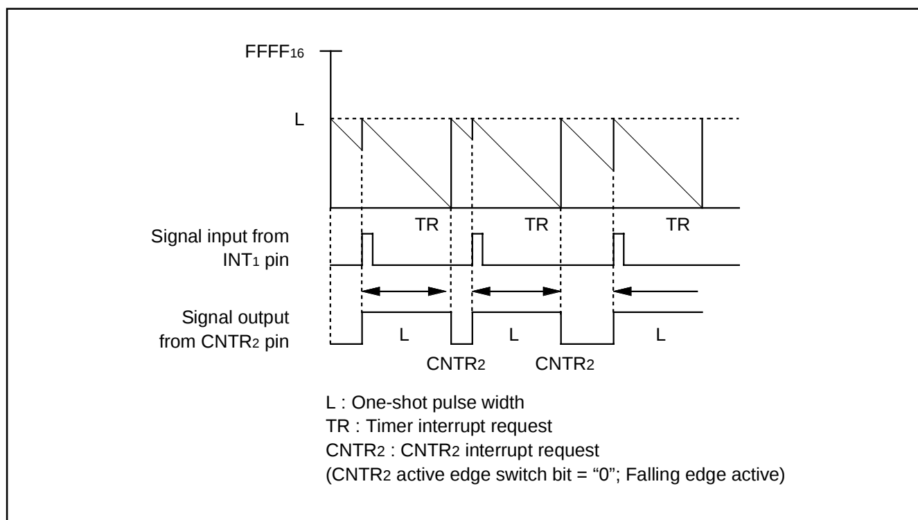
Fig. 39 Timing chart of programmable one-shot generating mode (“H” one-shot pulse generating)
