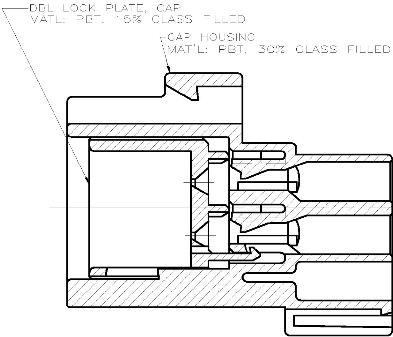
SECTION Z-Z SCALE 4:1
