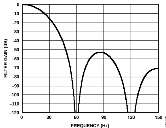
Figure 32. Sinc 4 Filter Response (FS[9:0] = 80)
