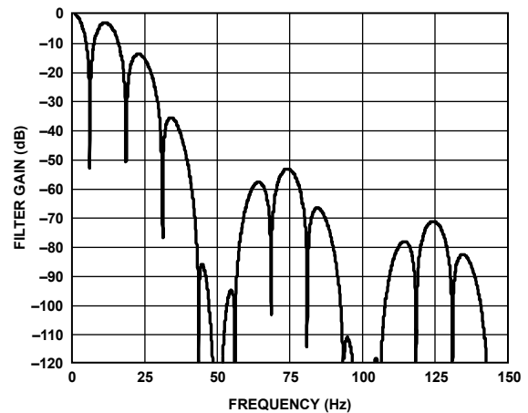
Figure 46. Sinc 4 Filter Response (FS[9:0] = 96, Chop Enabled)
