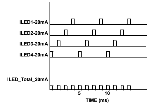
FIGURE 22. ISL97692 PHASE SHIFT 4-CHANNELS LED DRIVER WITH 10% PWM DIMMING CHANNEL CURRENT (UPPER) AND TOTAL CURRENT (LOWER)
