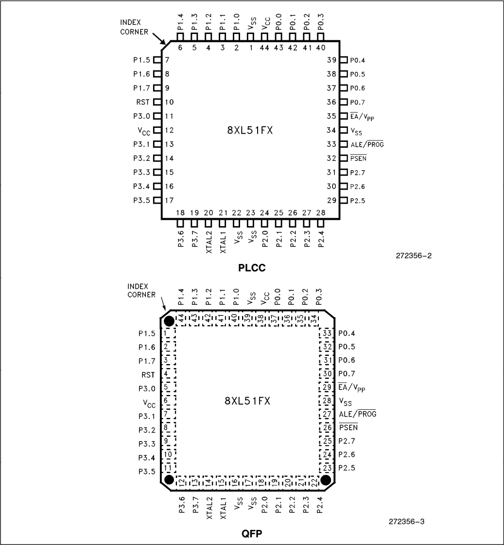
Figure 2. Pin Connections
