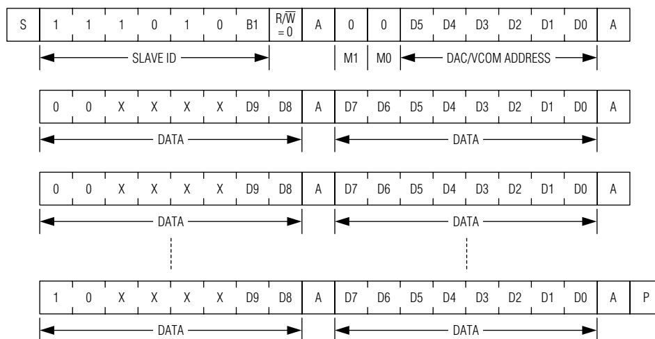
Figure 2. Multiple (or All) DACs Programming
