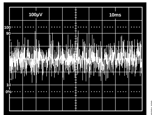
Figure 21. 1 Hz to 10 Hz Voltage Noise
