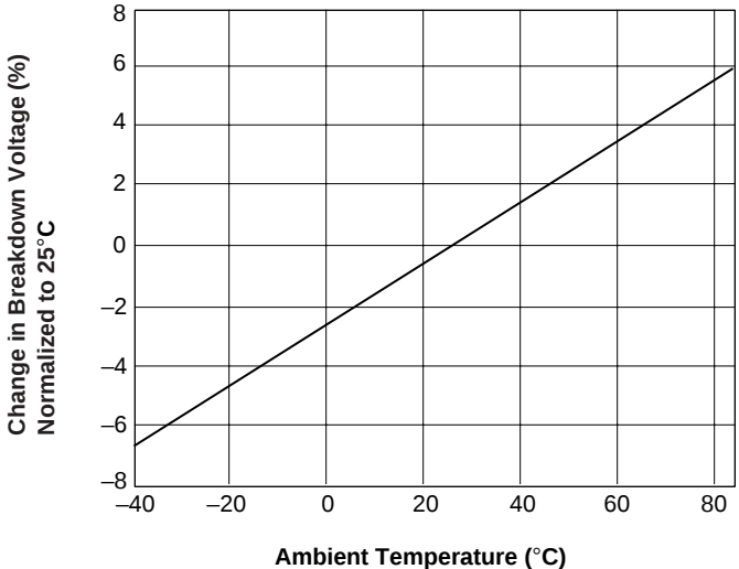
Figure 5. Switch Breakdown Voltage vs. Temperature
