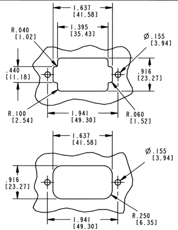
RECOMMENDED PANEL CUTOUTS
