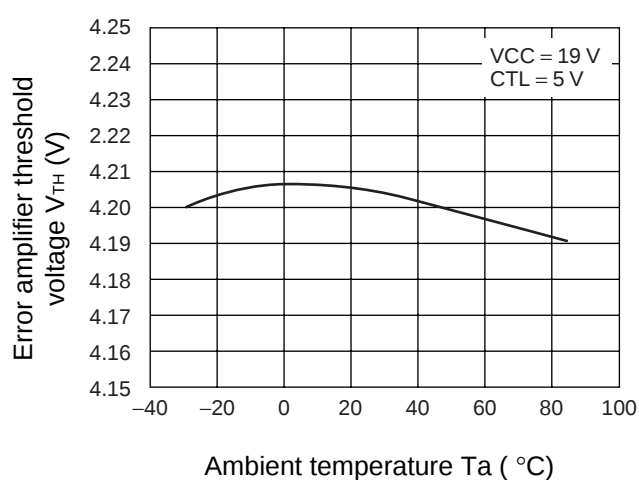
Error amplifier threshold voltage vs. Ambient temperature
