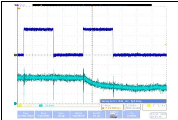
FIGURE 2-50: 100 kΩ – Low-Voltage Decrement Wiper Settling Time ( V_{DD} = 5.5\text{V} ) (1 μs/Div).
