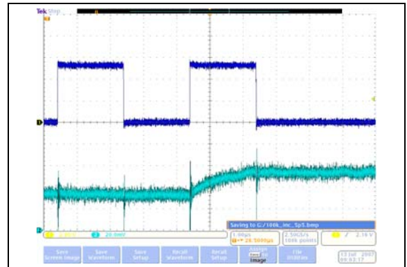
FIGURE 2-52: 100 kΩ – Low-Voltage Increment Wiper Settling Time ( V_{DD} = 2.7\text{V} ) (1 μs/Div).
