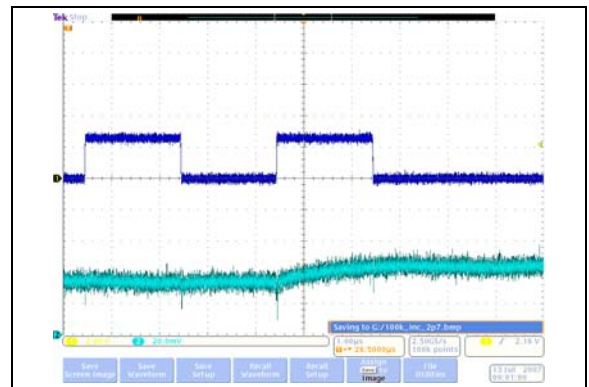
FIGURE 2-53: 100 kΩ – Power-Up Wiper Response Time (1 μs/Div).
