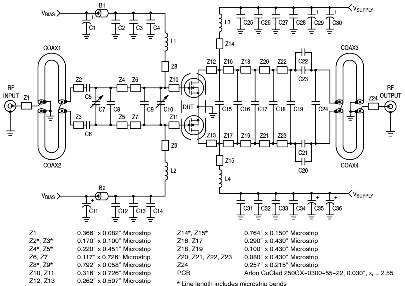
Figure 2. MMRF1006HR5(HSR5) Pulse Test Circuit Schematic — 450 MHz
