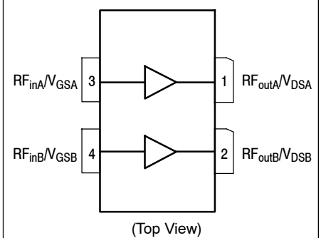
Figure 1. Pin Connections
