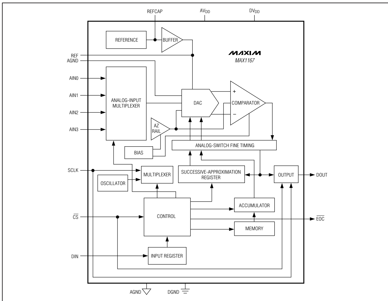
Figure 3. MAX1167 Functional Diagram
