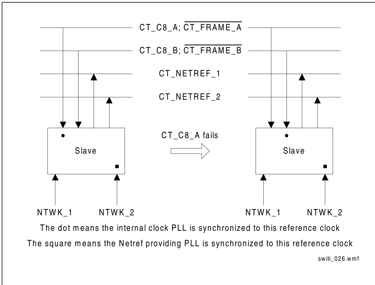
Figure 17 Clock Fallback of Slave
