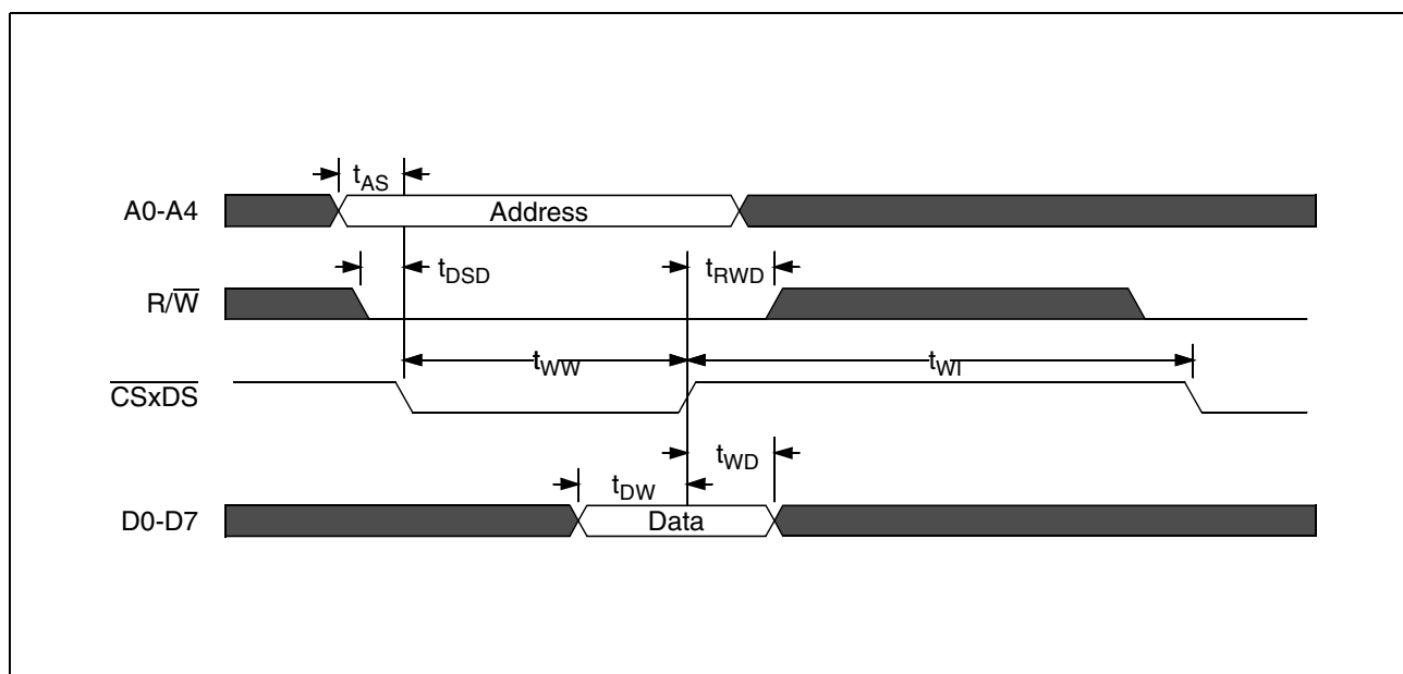
Figure 56 Motorola Write Cycle
