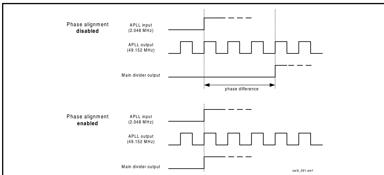
Figure 14 Example of Phase Alignment
