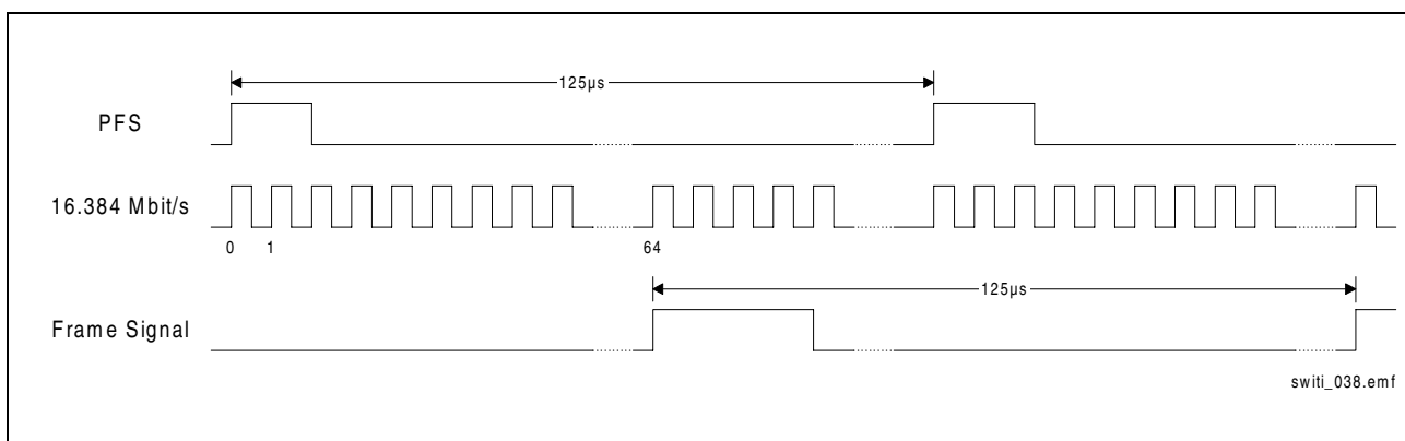
Figure 24 Frame Signal Example
