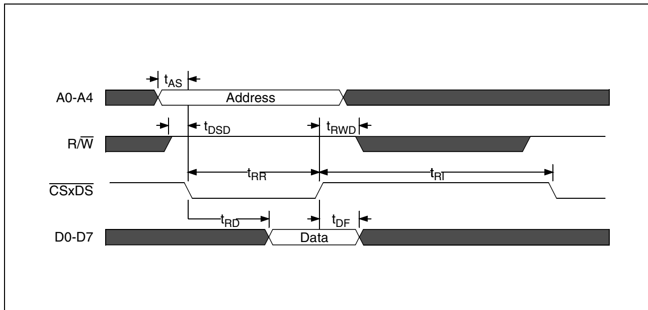
Figure 55 Motorola Read Cycle
