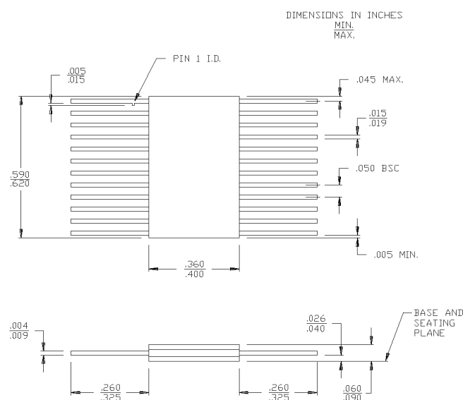
24-Lead Rectangular Cerpack K73 MIL-STD-1835 F-6 Config .A
