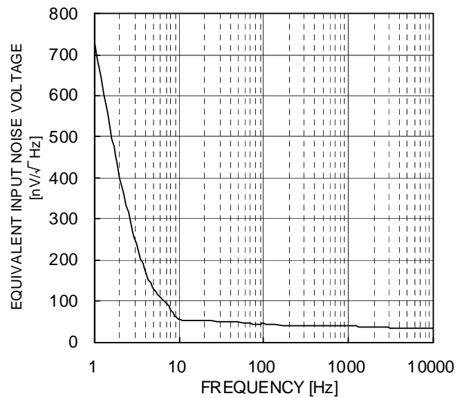
Figure 73. Input Referred Noise Voltage—Frequency (VDD/VSS=+2.5V/-2.5V, Av=0dB, Ta=25°C)
