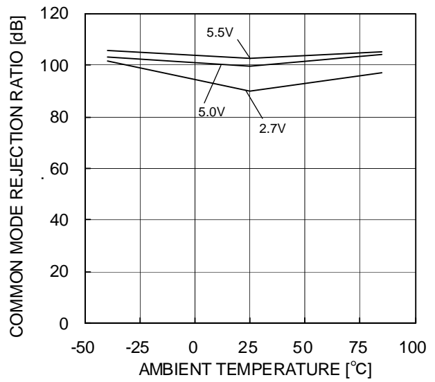
Figure 67. Common Mode Rejection Ratio – Ambient Temperature (VDD=3V)
