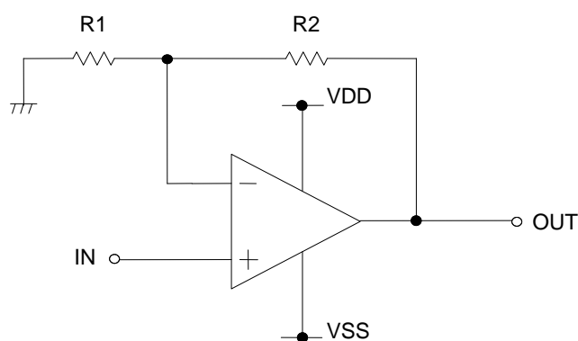
Figure 80. Non-inverting amplifier
