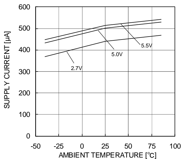
Figure 52. Supply Current – Ambient Temperature
