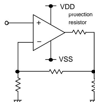
Figure 86. The example of output short protection
