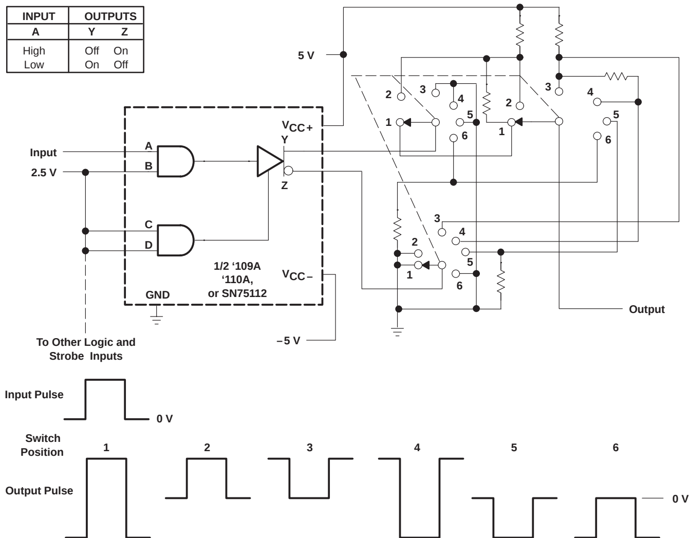
Figure 5. Pulse-Control Circuit
