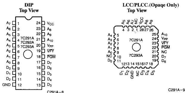
Figure 1. Programming Pinouts
