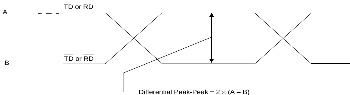
Figure 11. Differential V_{pp} of Transmitter or Receiver
