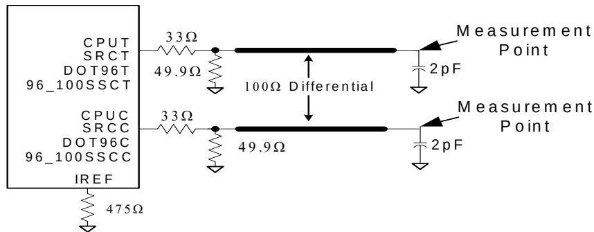
Figure 15. 0.7V Differential Clock Load Configuration
