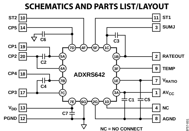
Figure 1. EVAL-ADXRS642 Schematic
