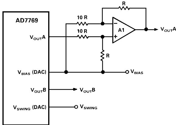
Figure 25. Increasing the DAC Output Voltage Resolution
