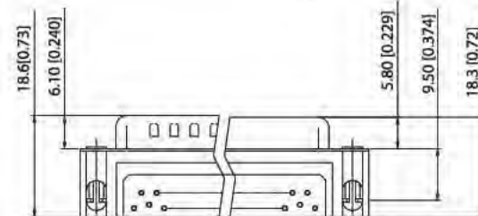
7.2mm[0.28"] Footprint
