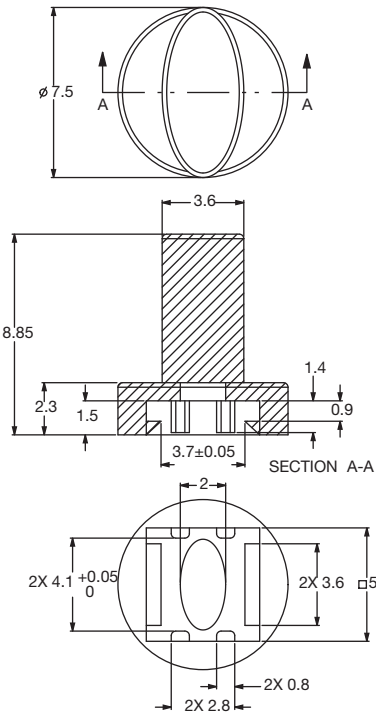
401E cap dimensions shown are “as molded” (no paint).
