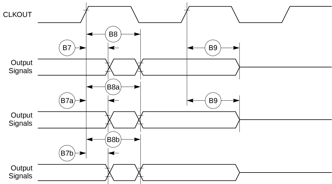
Figure 7. Synchronous Output Signals Timing
