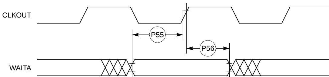
Figure 29. PCMCIA \overline{WAITA} Signals Detection Timing
