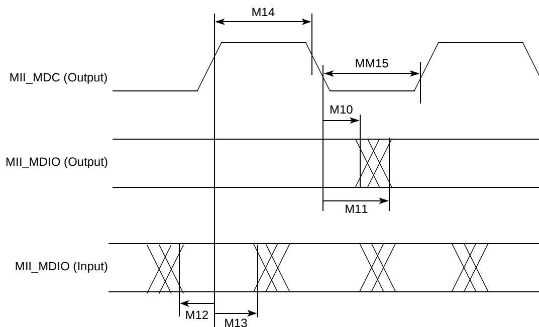
Figure 68. MII Serial Management Channel Timing Diagram
