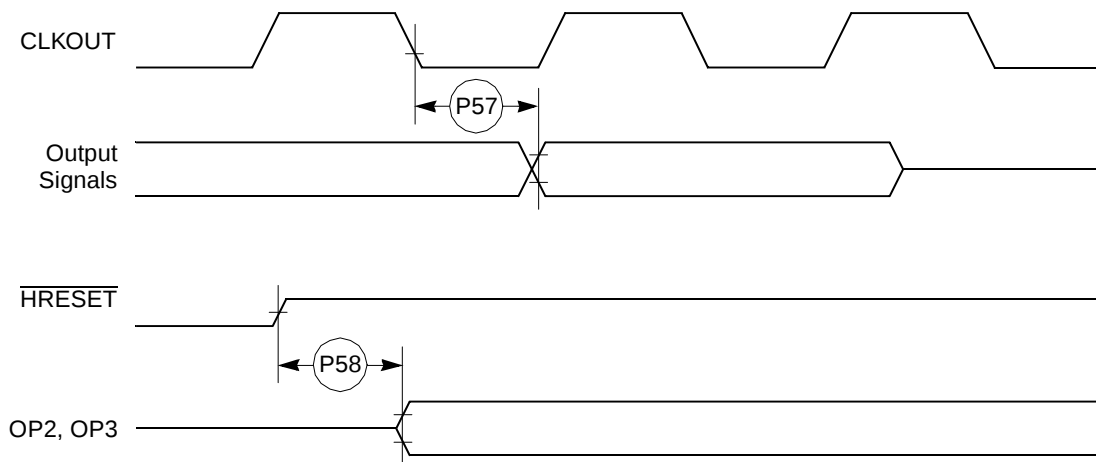
Figure 30. PCMCIA Output Port Timing
