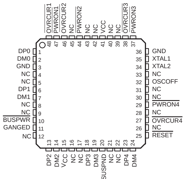
PT PACKAGE (TOP VIEW)
