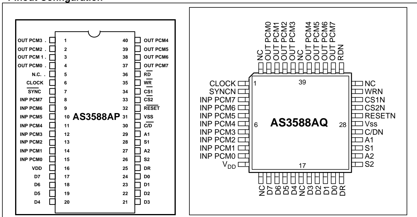
Figure 2: Pinout 40 pin DIP and 44 pin QFP
