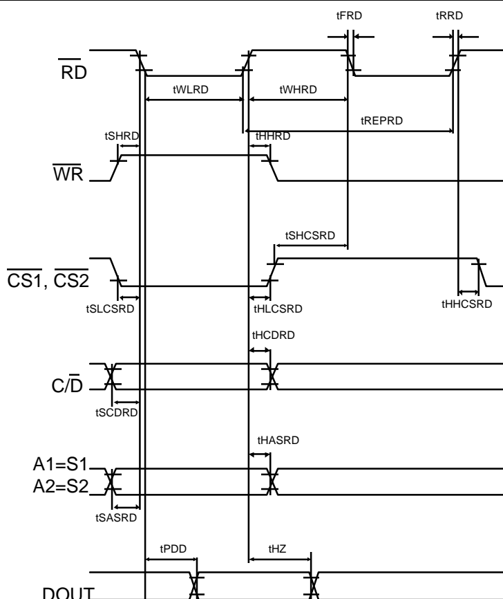
Figure 7 Read Timing
