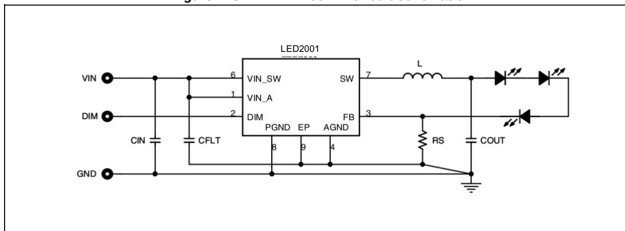
Figure 1. STEVAL-ILL054V1 circuit schematic
