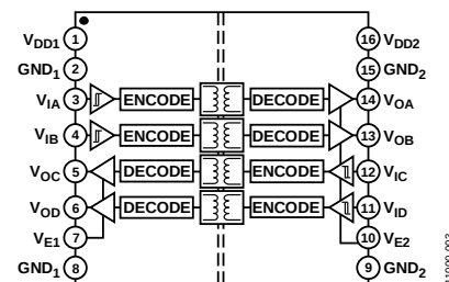
Figure 3. ADuM3402W Functional Block Diagram
