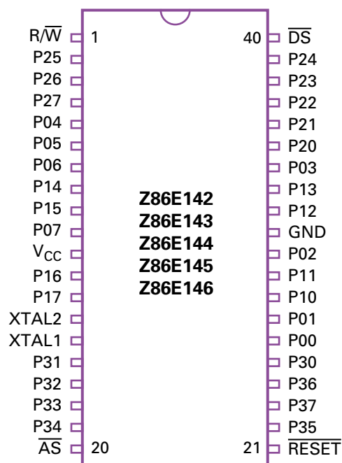
FIGURE 1. 40-PIN DIP CONFIGURATION
