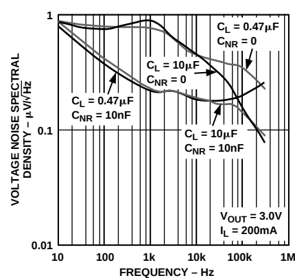
Figure 19. Output Noise Density
