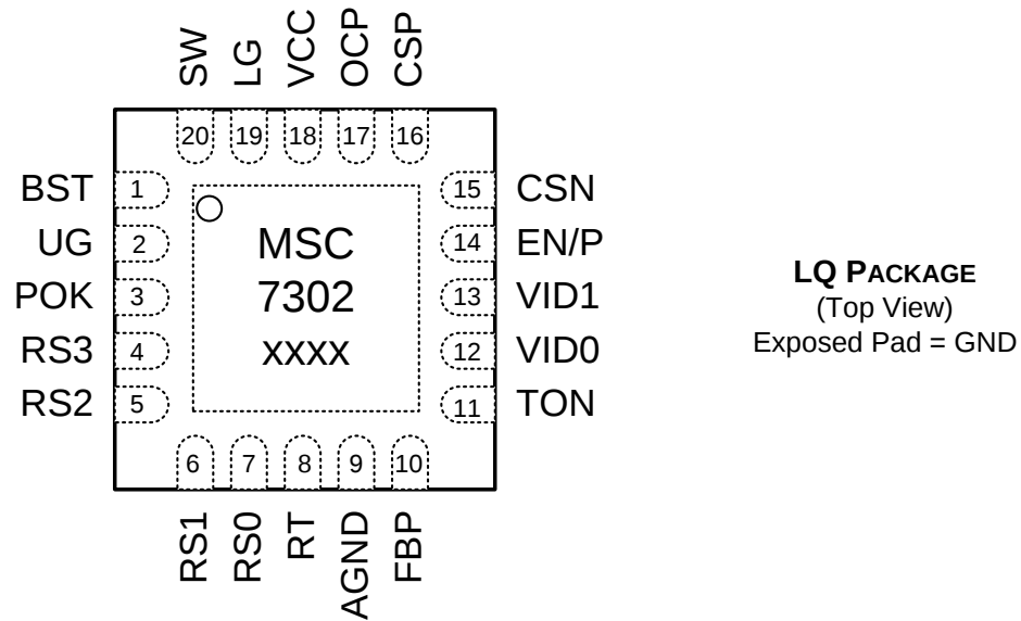
RoHS / Pb-free 100% Matte Tin Finish Figure 3: Pinout
