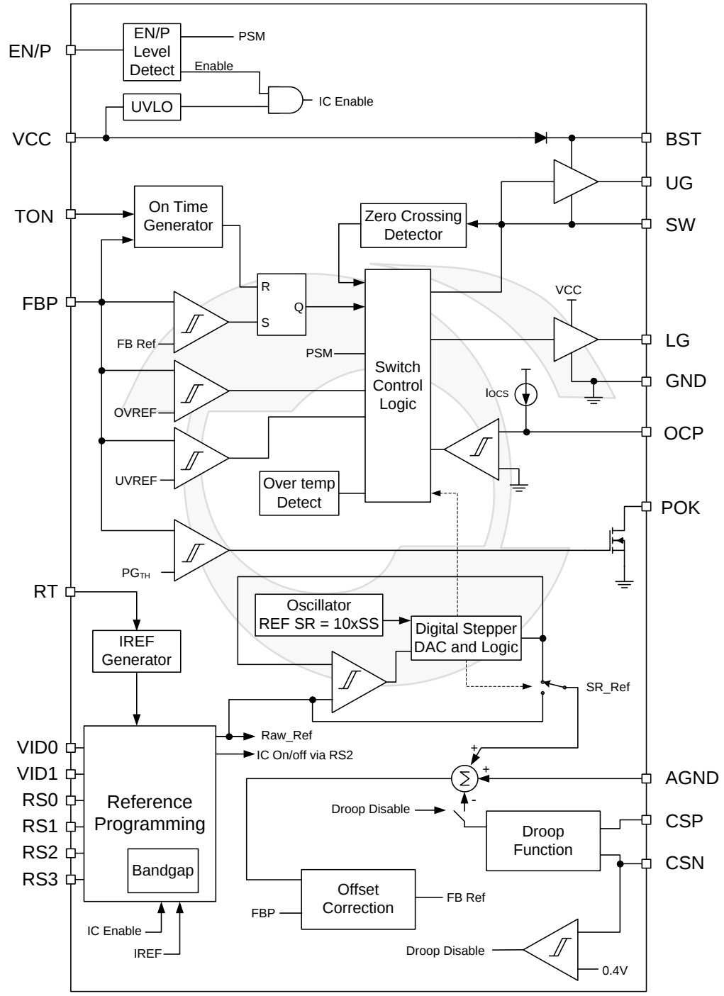
Figure 4: Block Diagram
