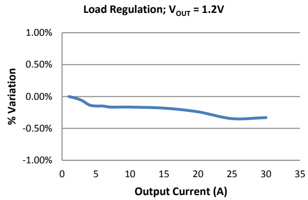
Figure 10. Load Regulation
