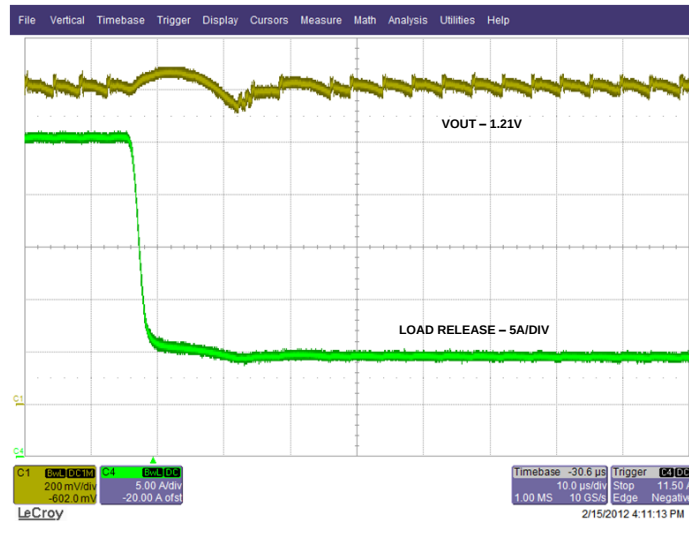
Figure 12. Transient Response – Load Release
