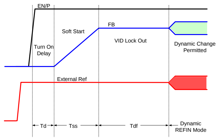
Figure 6. REFIN Power On Timing – Case 1
