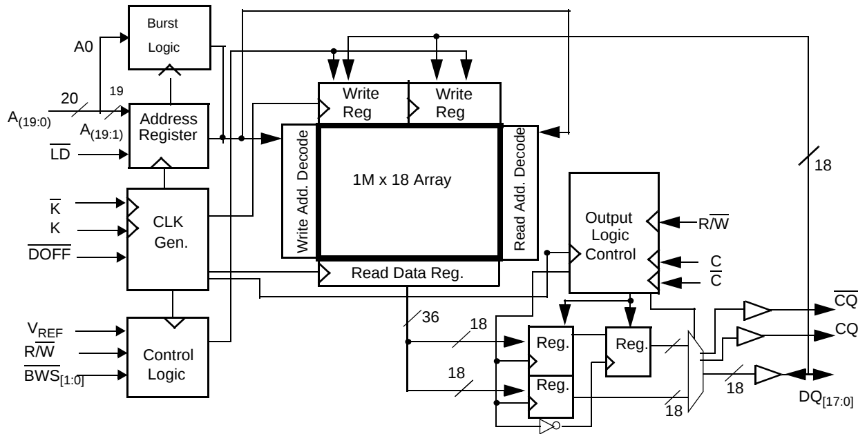
Logic Block Diagram (CY7C1318CV18)
