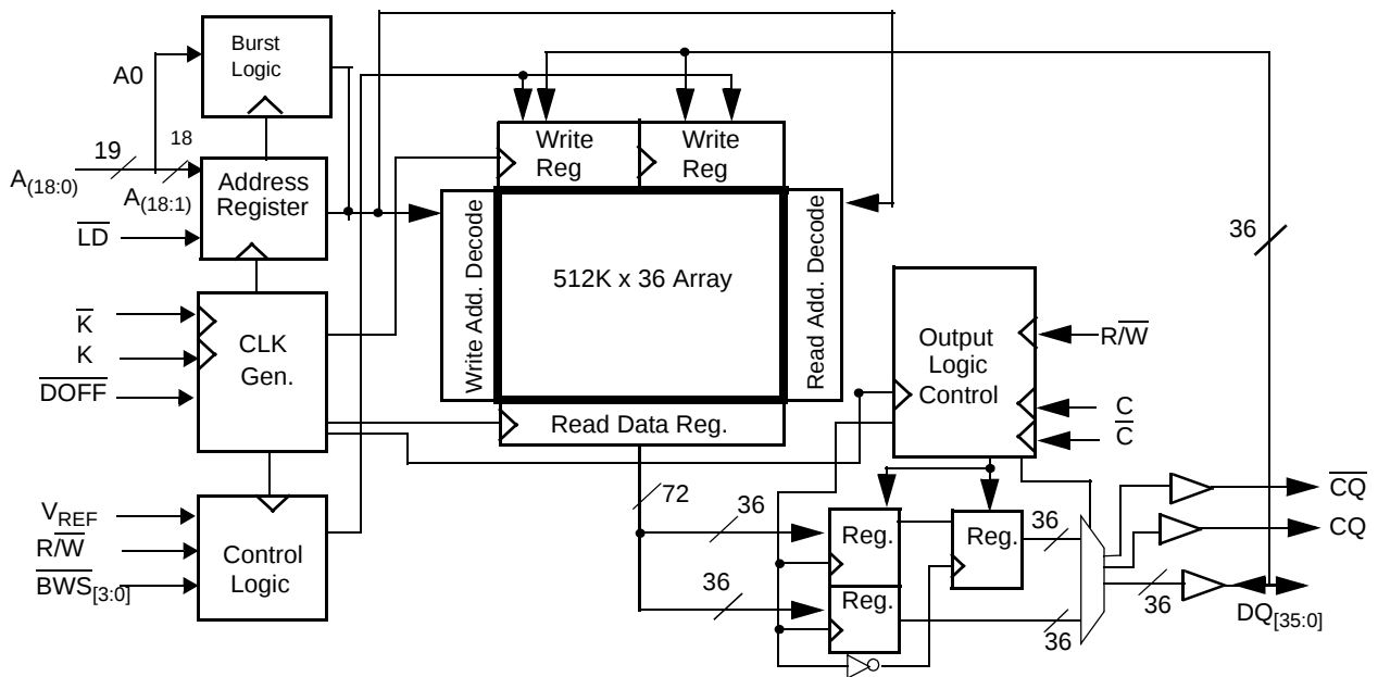
Logic Block Diagram (CY7C1320CV18)
