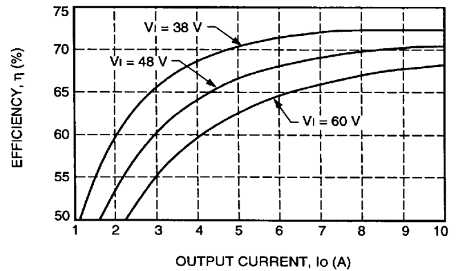
Figure 3. Typical FE050D Efficiency vs. Output Current at Room Temperature
