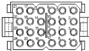
Plug
