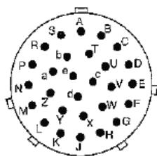
Shell Size 20
