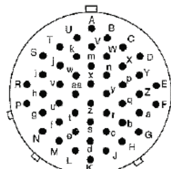
Shell Size 24
