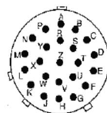
Shell Size 18
