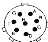
Shell Size 12
