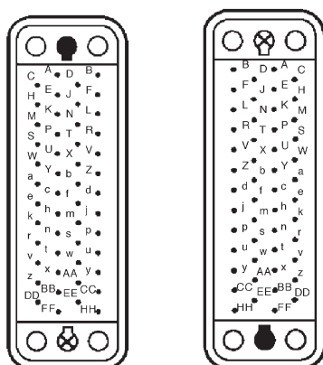
Plug Receptacle
