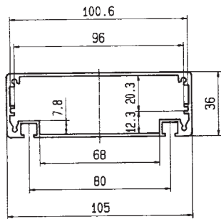
Enclosure Profile
