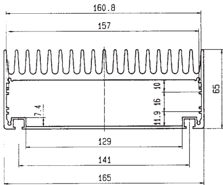
Enclosure Profile
