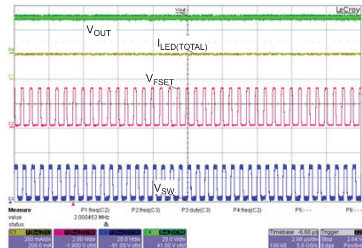
Figure 10: Synchronized FSET Pin and Switch Node SW Voltage.
