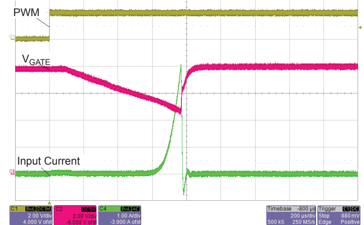
Figure 33: Startup into Output Shorted to GND fault. Input OCP tripped at 4 A ( R_{SC} = 0.024 \text{ W} , R_{adj} = 383 \Omega )
