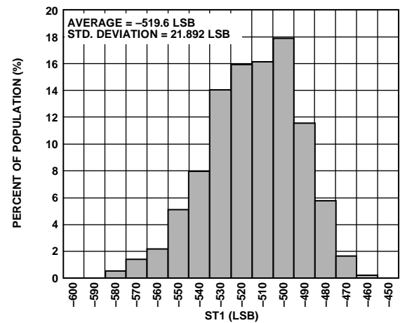
Figure 10. Self-Test 1 Histogram
