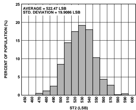
Figure 11. Self-Test 2 Histogram
