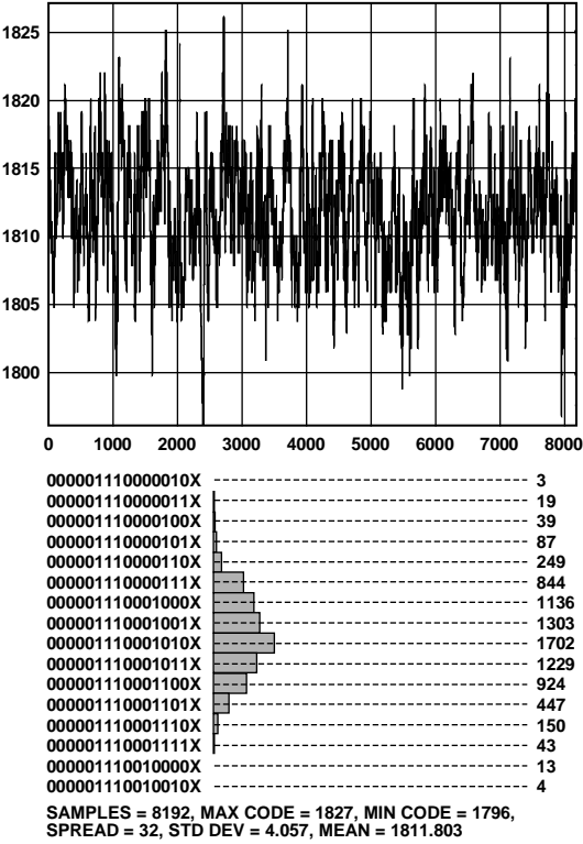
Figure 19. Noise Histogram
