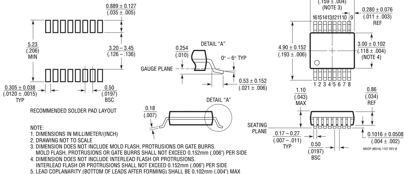
MS Package 16-Lead Plastic MSOP (Reference LTC DWG # 05-08-1669 Rev 0)
