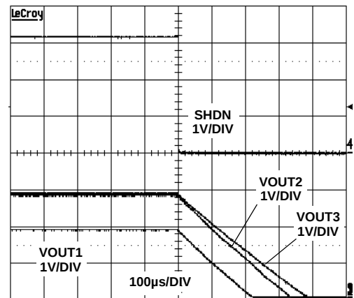
FIGURE 2. SHUTDOWN SEQUENCE
