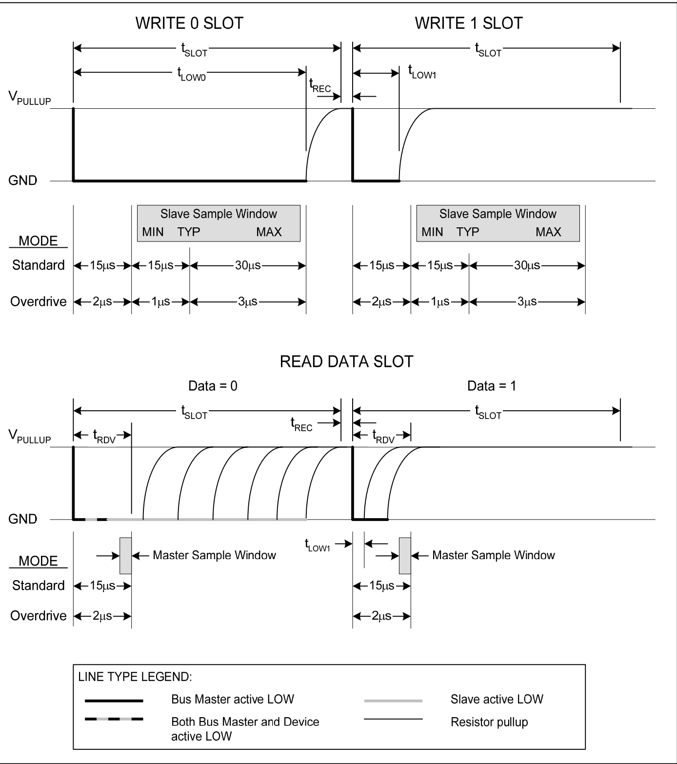
Figure 9. 1-Wire Write and Read-Time Slots
