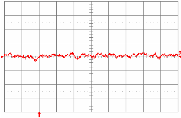
Fig. 1.2V.12: Input reflected ripple current, i_s (10 mA/div), measured through 10\ \mu\text{H} at the source at full rated load current and V_{in} = 48\ \text{V} . Refer to Fig. 1.2V.11 for test setup. Time scale: 1\ \mu\text{s}/\text{div} .
