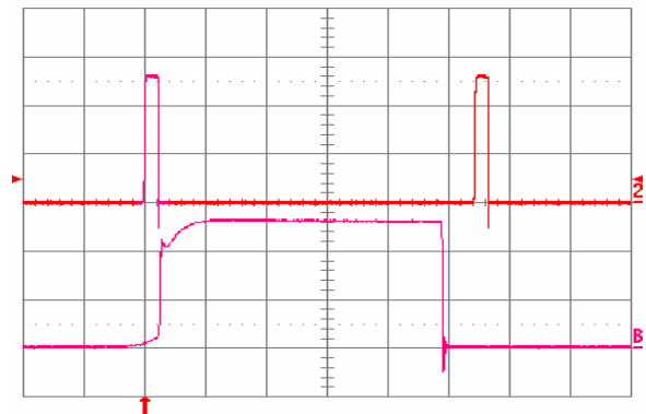
Fig. 1.2V.15: Load current (top trace, 20 A/div, 20 ms/div) into a 10\ \text{m}\Omega short circuit during restart, at V_{in} = 48\ \text{V} . Bottom trace (20 A/div, 1 ms/div) is an expansion of the on-time portion of the top trace.
