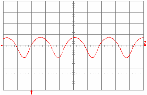
Fig. 1.2V.13: Input reflected ripple current, i_c (100 mA/div), measured at input terminals at full rated load current and V_{in} = 48\ \text{V} . Refer to Fig. 1.2V.11 for test setup. Time scale: 1\ \mu\text{s}/\text{div} .
