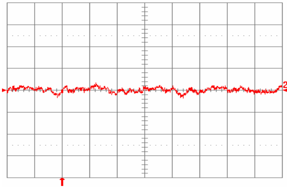
Fig. 2.5V.12: Input reflected ripple current, i_s (10 mA/div), measured through 10 \mu H at the source at full rated load current and V_{in} = 48 V. Refer to Fig. 2.5V.11 for test setup. Time scale: 1 \mu s/div.
