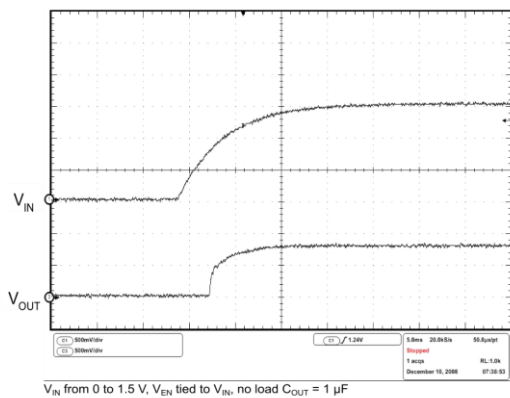
Figure 16: Start-up transient
