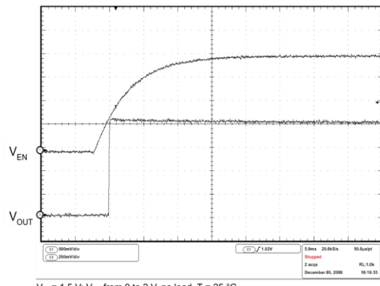
Figure 17: Enable transient
