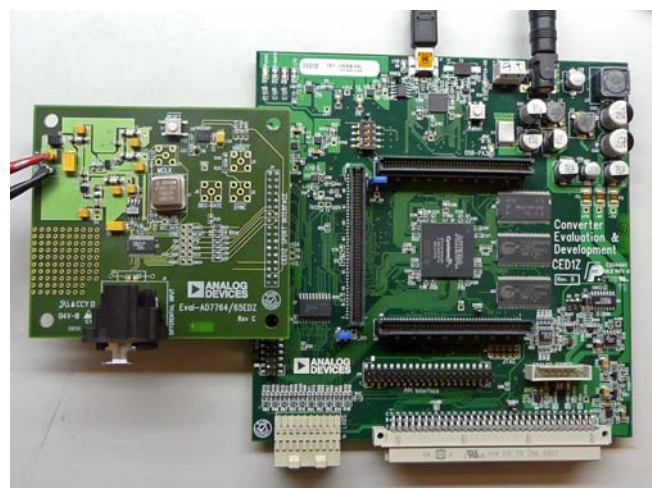
Figure 10. Connecting the EVAL-AD7764/AD7765 board to EVAL-CED1Z.
