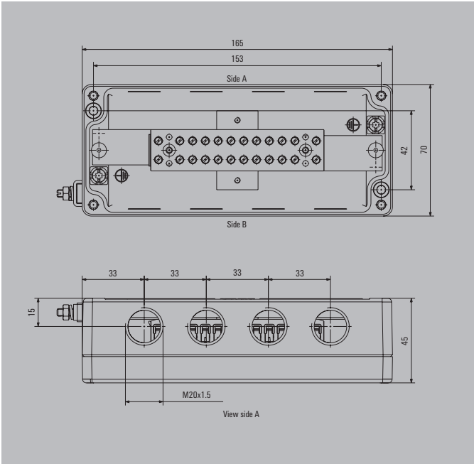
Height / Width / Depth 70 / 165 / 45 mm
